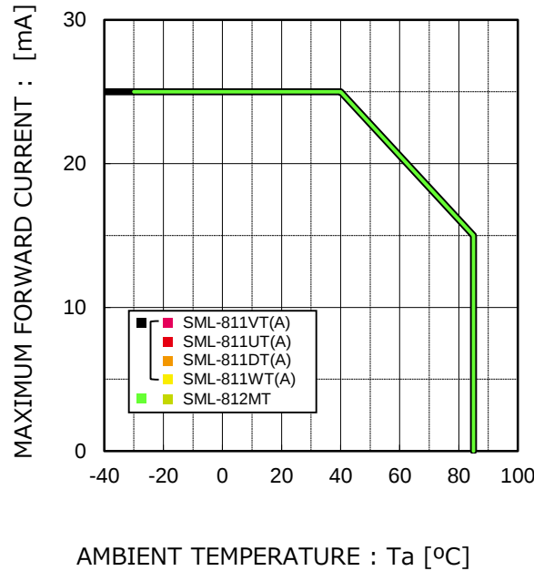
Fig.4 Derating
