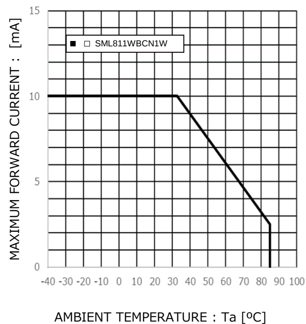
Fig.4 Derating
