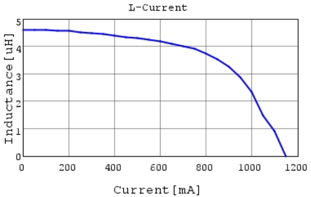
LQH2MPZ4R7MGR L-Current 20degC
