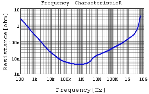
GRM185R60J106ME15 R DCOV, 25degC
