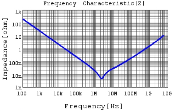
GRM185R60J106ME15 |Z| DCOV, 25degC
