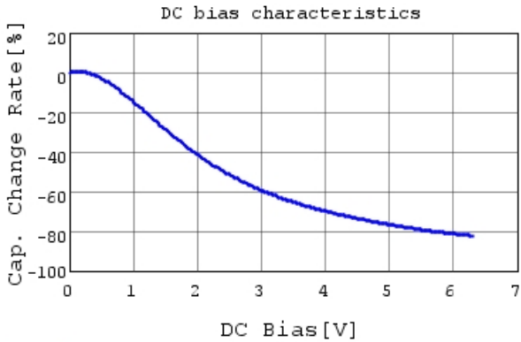
GRM185R60J106ME15 C-DC bias capchange, 25.0c
