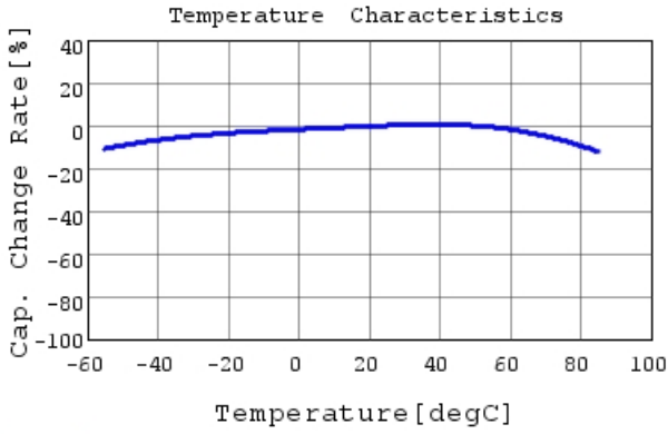
GRM185R60J106ME15 C-Temp. capchange, DC0.0V,
