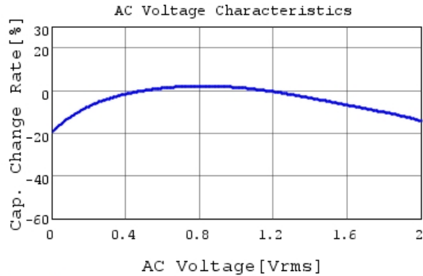
GRM185R60J106ME15 C-AC Voltage capchange, DC
