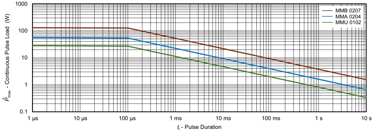
Maximum pulse load, continuous pulse; applicable if \hat{P} \leq P(\vartheta_{amb}) and \hat{U} \leq \hat{U}_{max} ; for permissible resistance change \pm (0.5\% R + 0.01 \Omega)
