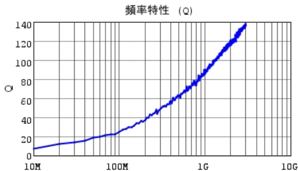
LQP03HQ1N3W02 Q
