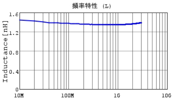
LQP03HQ1N3W02 L
