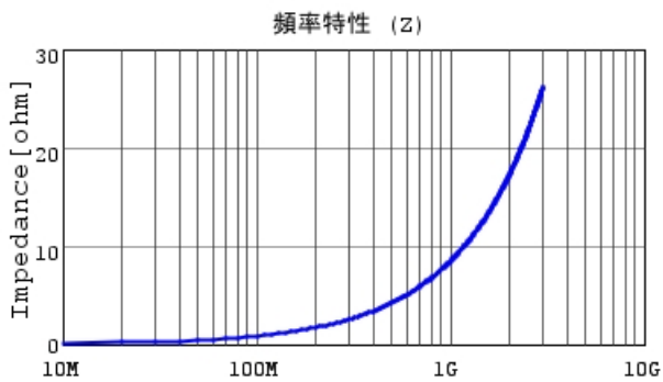
LQP03HQ1N3W02 |Z|
