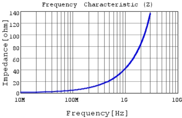
LQP02TN6N8H02 |Z|
