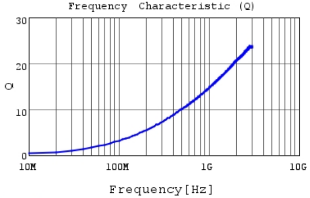
LQP02TN6N8H02 Q
