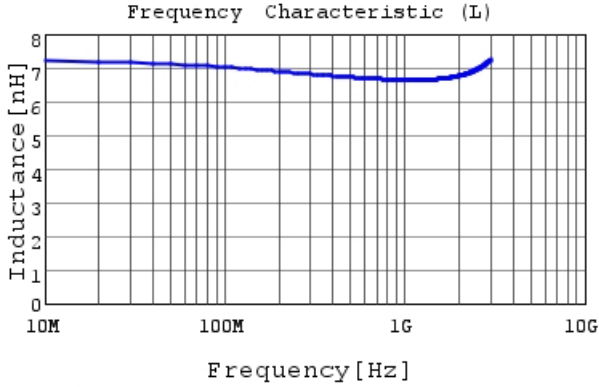
LQP02TN6N8H02 L
