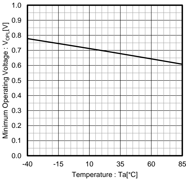
Figure 9. Minimum Operating Voltage vs Temperature (V OUT Pull-up to 5 V, R L = 100 kΩ)
