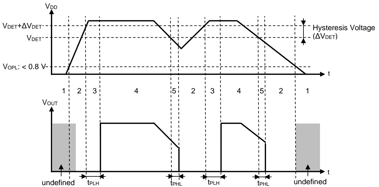
Figure 19. Timing Diagram
