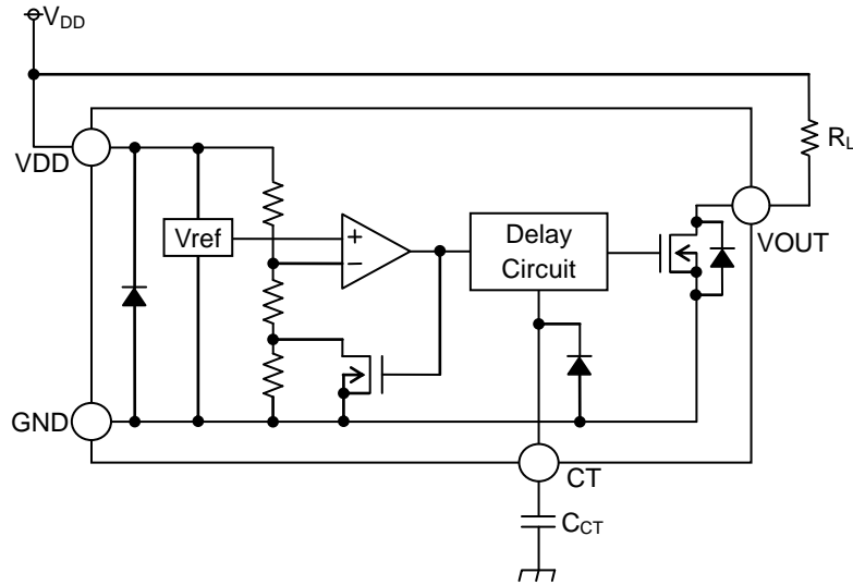
Figure 18. BD52xxG-1 Set-up
