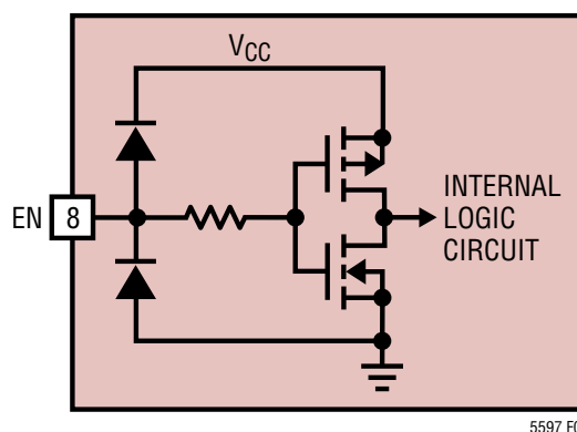
Figure 7. Simplified Schematic of the EN Interface
