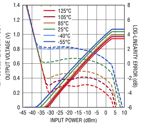
Output Voltage, Linearity Error vs RF Input Power at 70GHz
