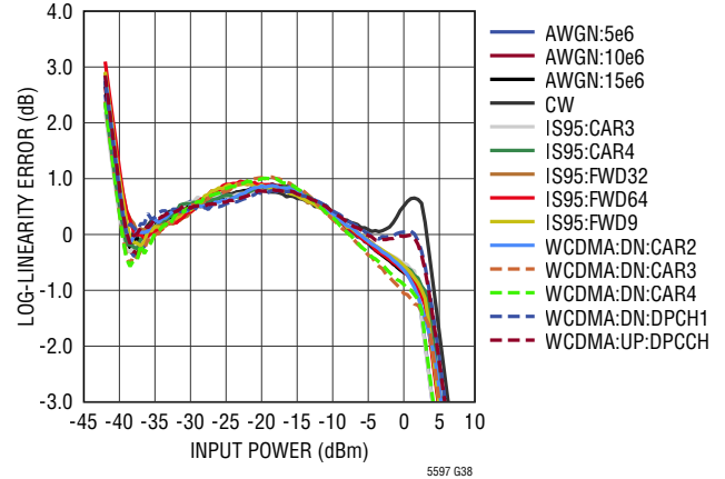
Linearity Error vs RF Input Power for Various Modulation Formats, Regression Using CW Slope and Intercept Values
