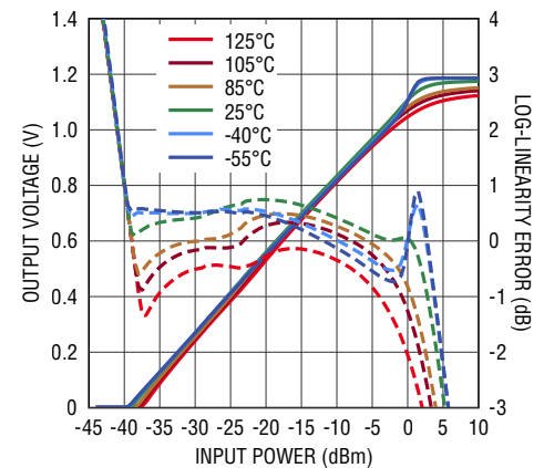
Output Voltage, Linearity Error vs RF Input Power at 52GHz
