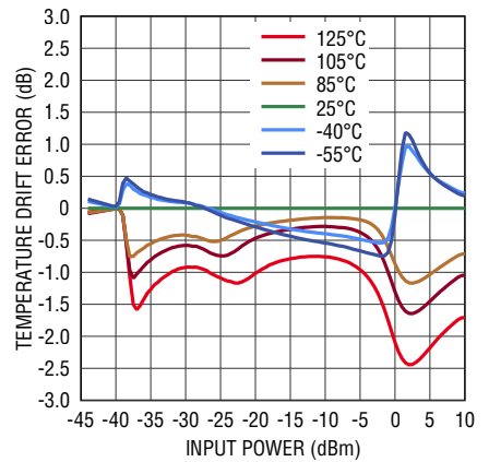
Linearity Error Temperature Variation from 25^\circ C at 52GHz
