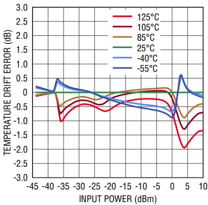
Linearity Error Temperature Variation from 25^\circ C at 42GHz
