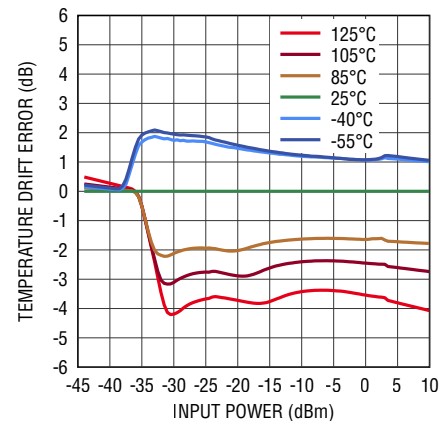
Linearity Error Temperature Variation from 25^\circ C at 70GHz
