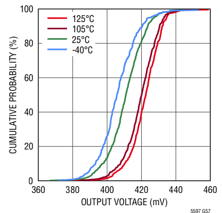
Output Voltage at -25dBm Cumulative Distribution
