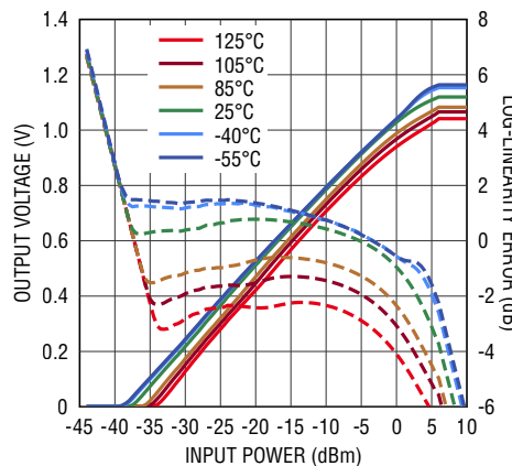
Output Voltage, Linearity Error vs RF Input Power at 67GHz
