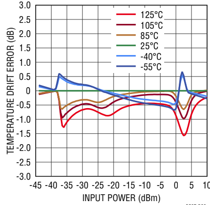
Linearity Error Temperature Variation from 25^\circ C at 30GHz
