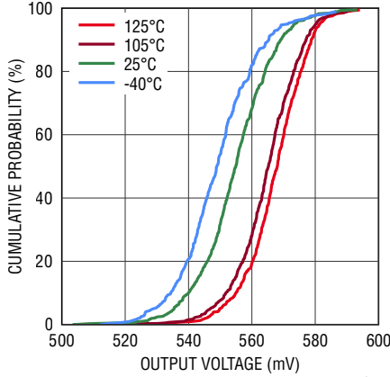
Output Voltage at -20dBm Cumulative Distribution
