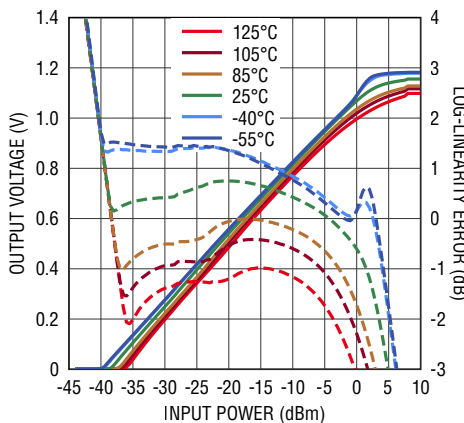
Output Voltage, Linearity Error vs RF Input Power at 60GHz
