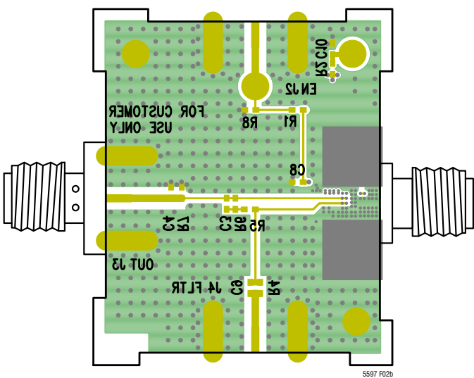
Figure 2b. Bottom Side of Evaluation Board
