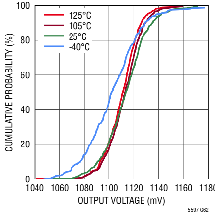
Output Voltage at 0dBm Cumulative Distribution
