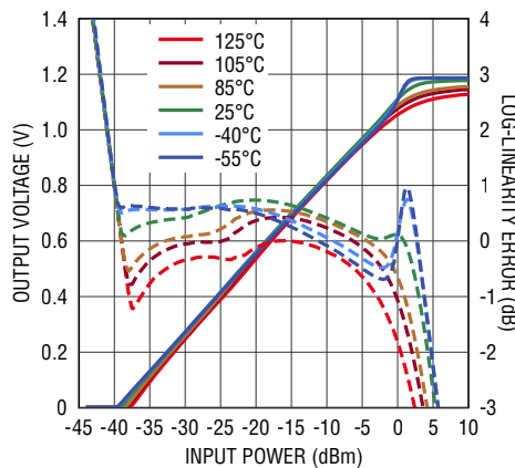
Output Voltage, Linearity Error vs RF Input Power at 50GHz
