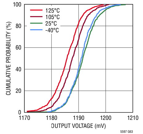
Output Voltage at 5dBm Cumulative Distribution
