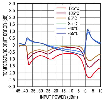
Linearity Error Temperature Variation from 25^\circ C at 50GHz
