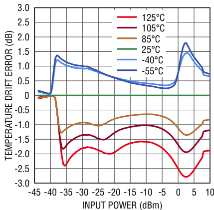
Linearity Error Temperature Variation from 25^\circ C at 60GHz
