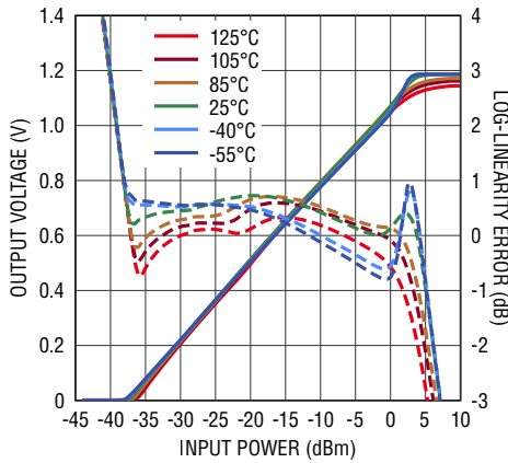
Output Voltage, Linearity Error vs RF Input Power at 42GHz
