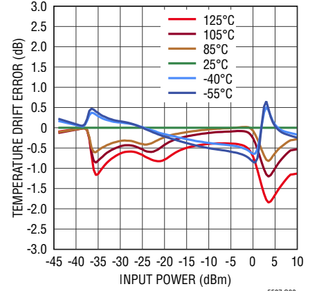
Linearity Error Temperature Variation from 25^\circ C at 39GHz
