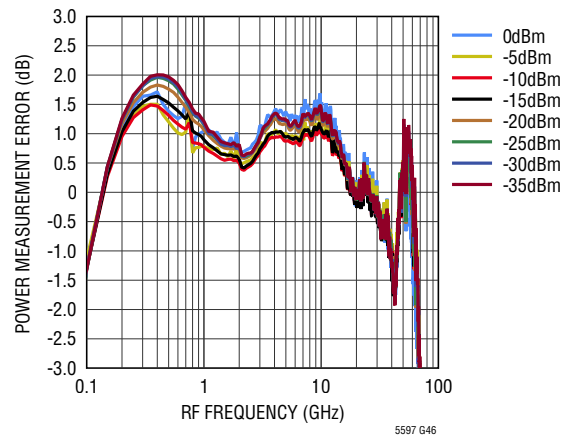
Power Measurement Error vs Frequency, Relative to Response at 18GHz
