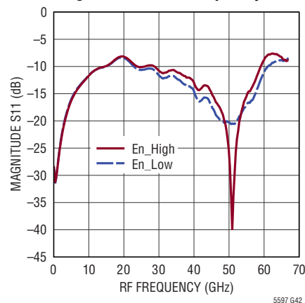
Magnitude S11 vs Frequency
