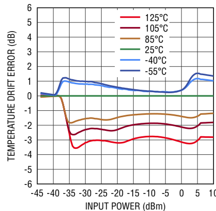
Linearity Error Temperature Variation from 25^\circ C at 67GHz
