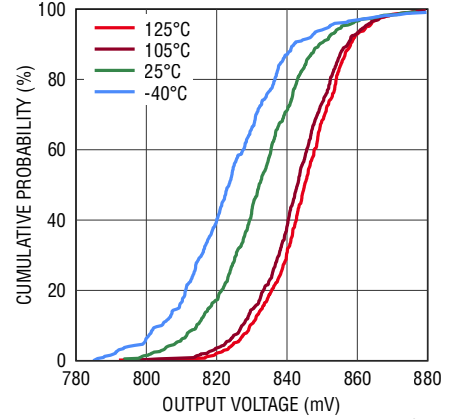
Output Voltage at -10dBm Cumulative Distribution
