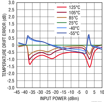
Linearity Error Temperature Variation from 25^\circ C at 28GHz
