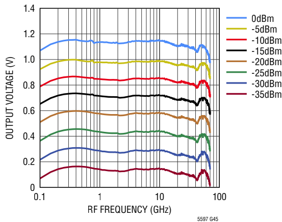
Output Voltage vs Frequency
