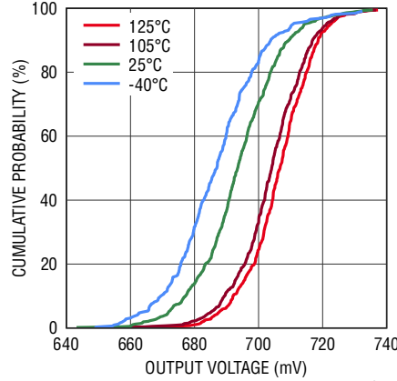
Output Voltage at -15dBm Cumulative Distribution
