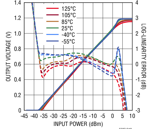
Output Voltage, Linearity Error vs RF Input Power at 39GHz
