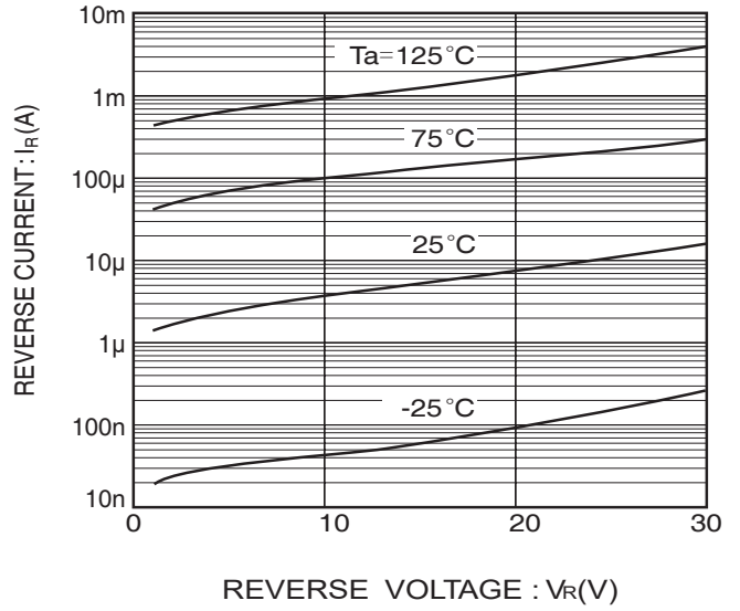
Fig. 2 Reverse characteristics
