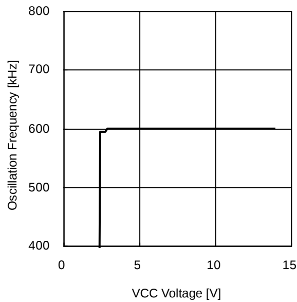
Figure 5. Oscillation Frequency vs V CC Voltage
