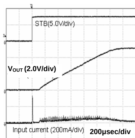
Figure 16. Starting Waveform Example of Application Circuit [2] ( L=10\mu\text{H} , C_{\text{OUT}} = 47\mu\text{F} , f_{\text{OSC}} = 750\text{ kHz} , unloaded)
