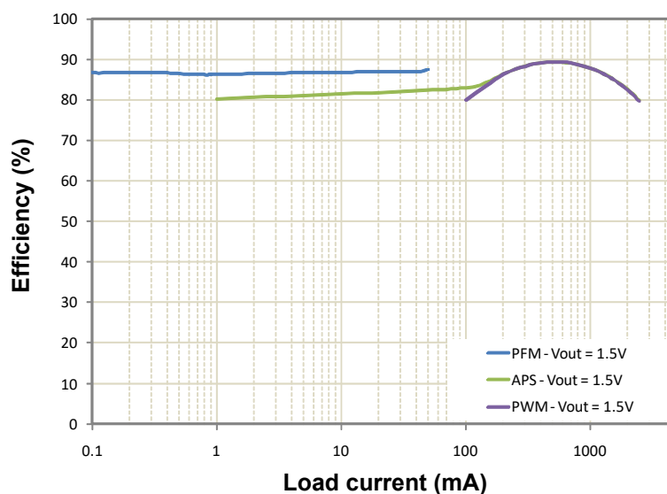
Figure 20. SW3AB single phase efficiency waveforms
