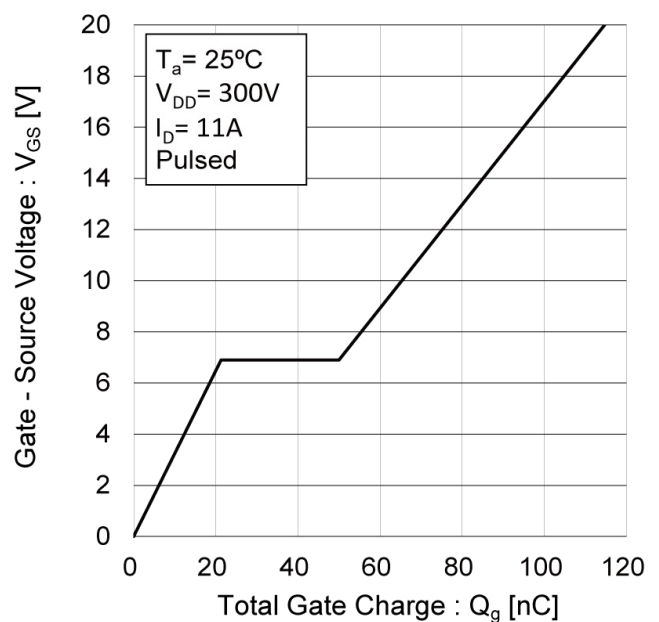
Fig.16 Gate charge
