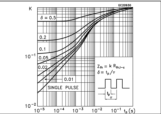
Figure 2. Thermal impedance for TO-220
