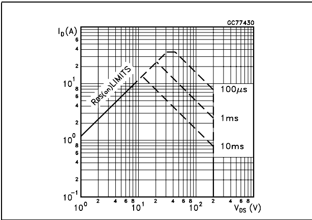
Figure 1. Safe operating area for TO-220
