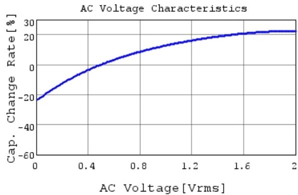
GRM31CR61C226ME15 C-AC Voltage capchange, Dc
