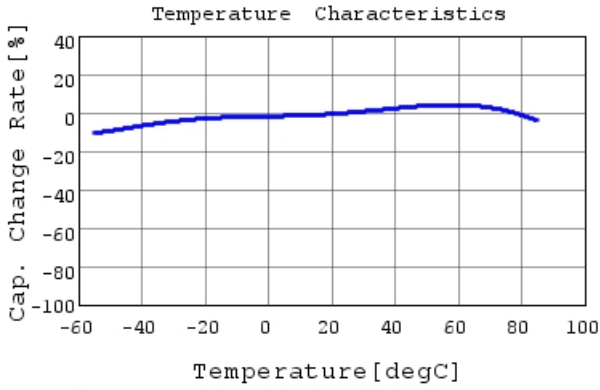
GRM31CR61C226ME15 C-Temp. capchange, DC0.0V,
