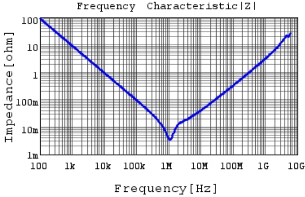
GRM31CR61C226ME15 |Z| DCOV,25degC
