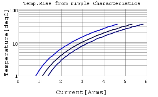
GRM31CR61C226ME15 Temp.rise — 80kHz —
