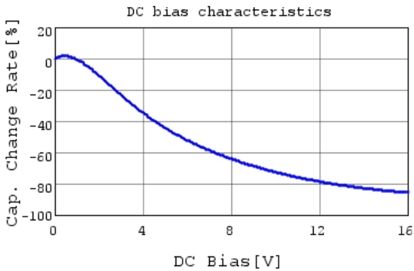
GRM31CR61C226ME15 C-DC bias capchange, 25.0c
