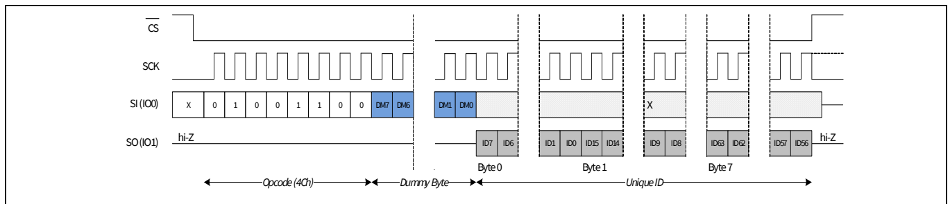
Figure 91 Read unique ID in SPI mode
