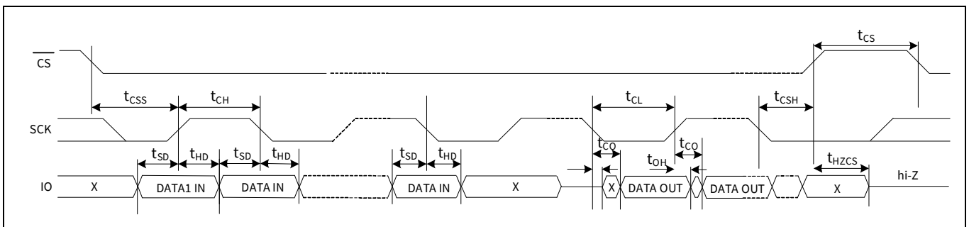
Figure 119 SPI switching timing - multiple I/O, DDR [30]
