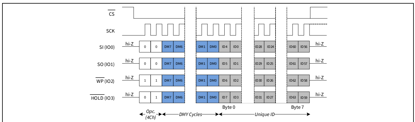
Figure 93 Read unique ID in QPI mode
