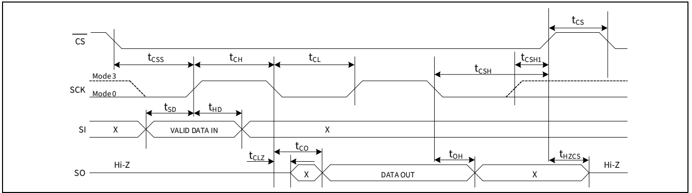
Figure 115 SPI switching timing - single IO, SDR (mode 0 and mode 3)
