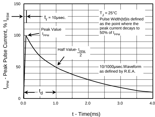
Pulse Waveform
