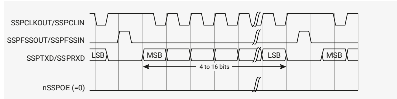
Figure 94. Motorola SPI frame format, continuous transfer, with SPO=1 and SPH=0
