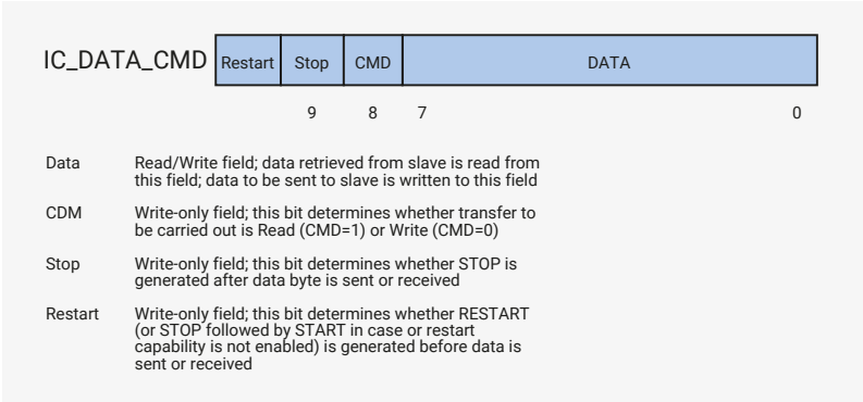
Figure 72. IC_DATA_CMD Register
