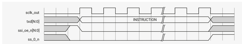
Figure 151. Instruction only transfer in enhanced SPI Format
