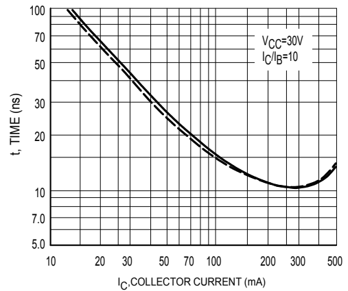
Figure 4. Rise Times
