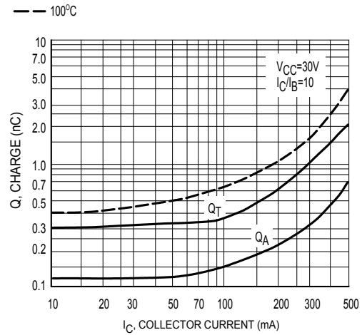
Figure 2. Charge Data
