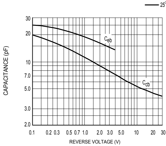
Figure 1. Capacitances
