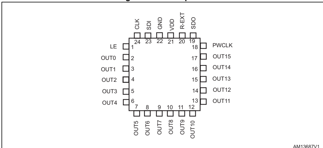
Figure 2. QFN-24 pinout
