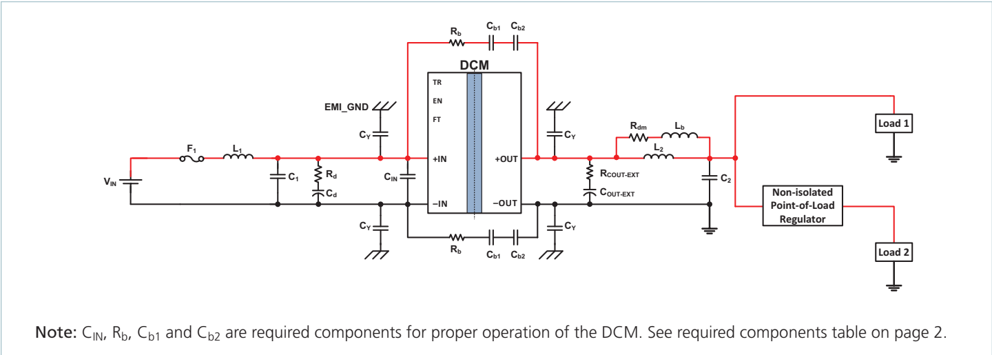
Single DCM2322x72S13A0y6z, to a non-isolated regulator, and direct to load
