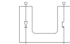
Internal connection diagram
