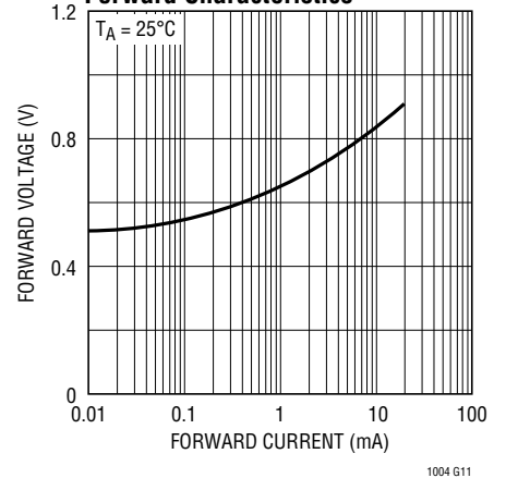
Forward Characteristics
