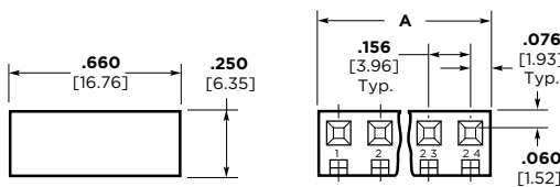
(C) Without Locking Ramp/Without Polarizing Tabs
