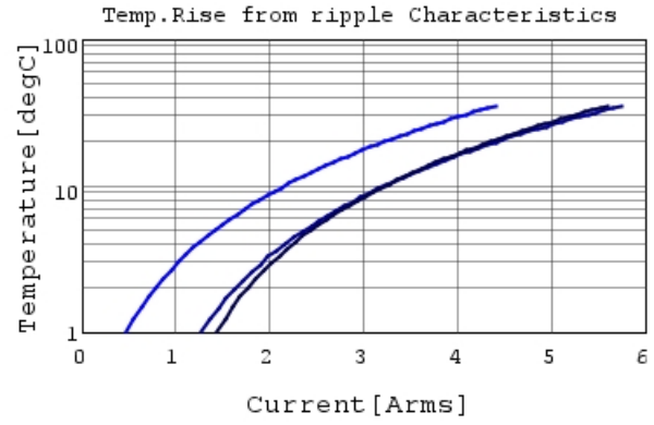
GRT21BR61A226ME13 Temp.rise — 80kHz —
