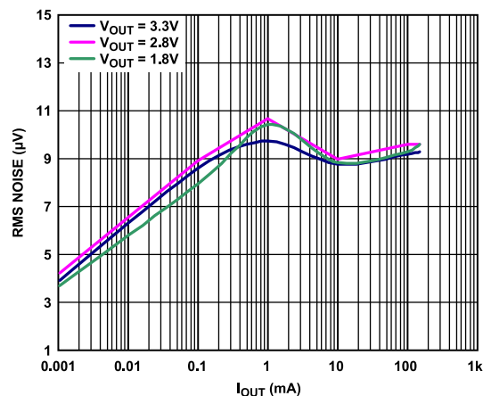
Figure 20. Output RMS Noise vs. Load Current ( I_{OUT} ) and Output Voltage ( V_{OUT} ), V_{IN} = 5V , C_{OUT} = 1\mu F
