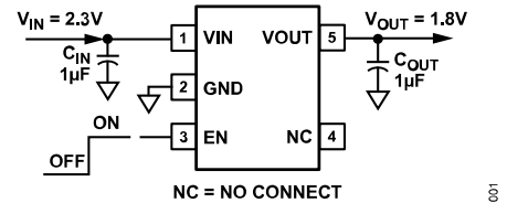
Figure 1. 5-Lead TSOT with Fixed Output Voltage, 1.8 V
