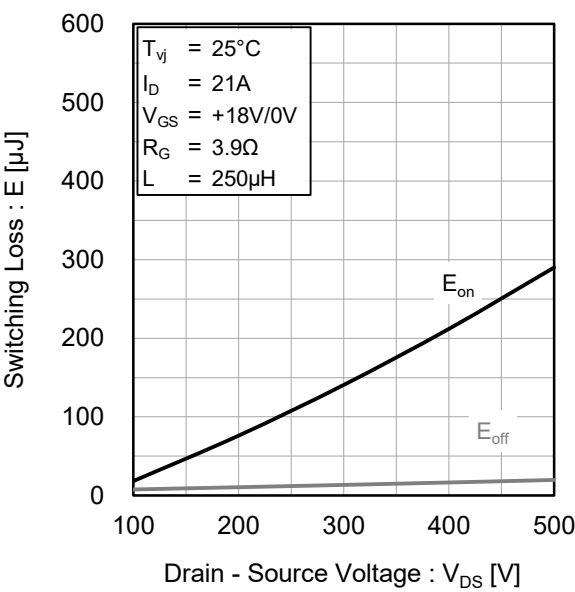
Fig.21 Typical Switching Loss vs. Drain - Source Voltage
