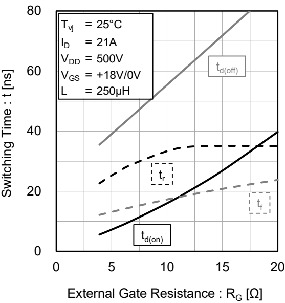
Fig.20 Typical Switching Time vs. External Gate Resistance
