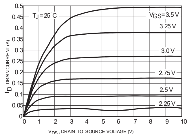
Fig2. On-Region Characteristics
