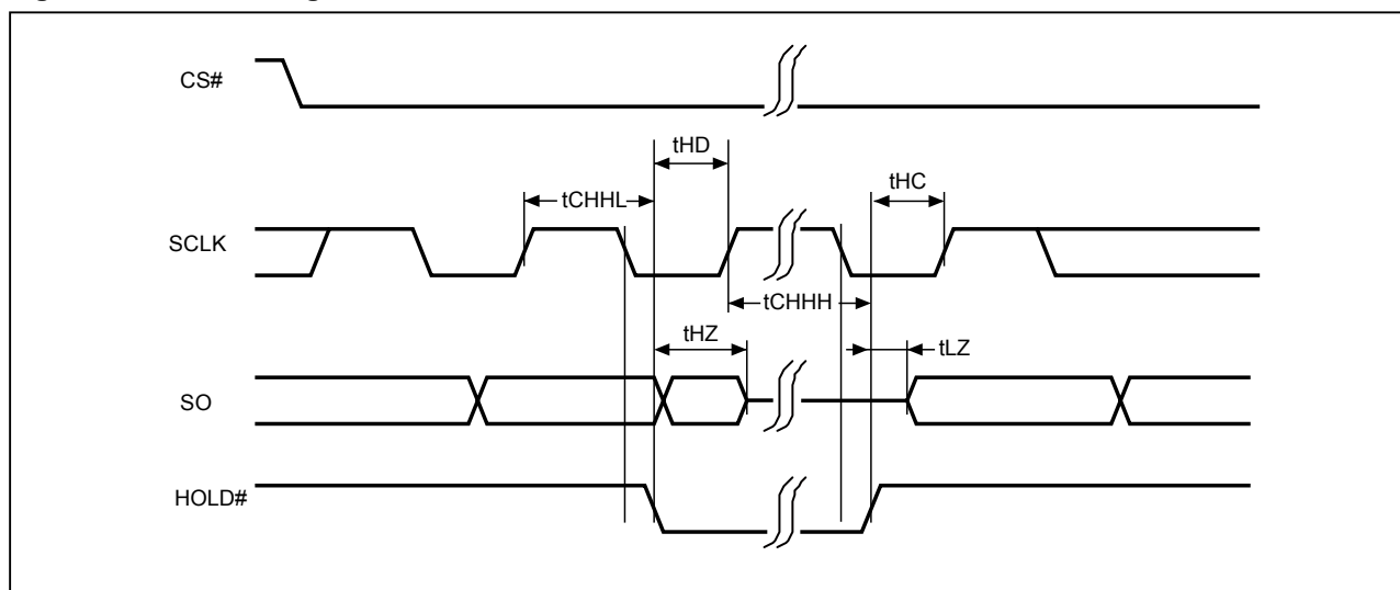
Figure 33. Hold Timing
