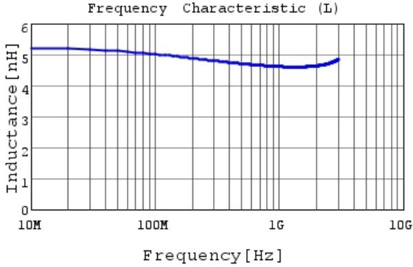
LQP02TN4N7H02 L
