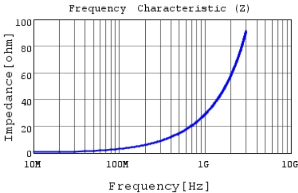
LQP02TN4N7H02 |Z|
