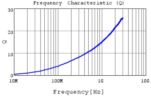
LQP02TN4N7H02 Q
