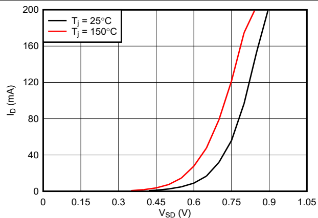
Figure 5-7. Source current as a function of source-drain voltage
