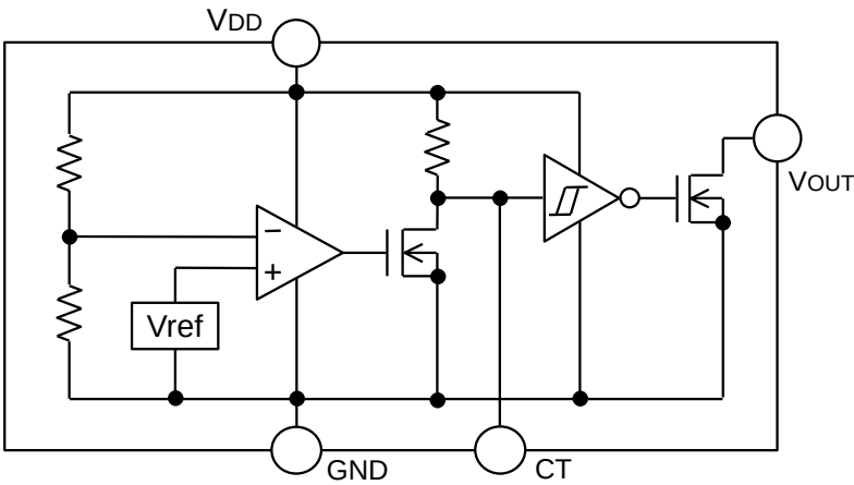
Figure.1 BD52Exxx-M Series
