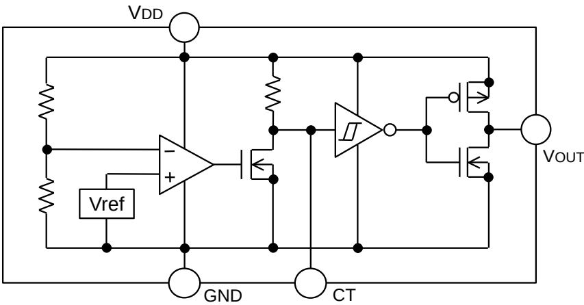
Figure.2 BD53Exxx-M Series
