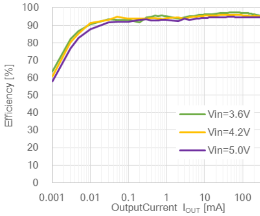
RP515x331x, Ta=25°C
