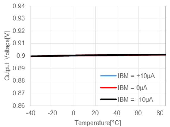
13) BM Output Voltage vs Temperature ( C_{OUT2} = Ceramic 0.1 \mu F, T_a = 25 ^{\circ} C) RP515xxx3x RP515xxx4x
