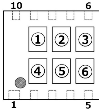
RP515K [DFN(PL)2527-10] Part Markings
