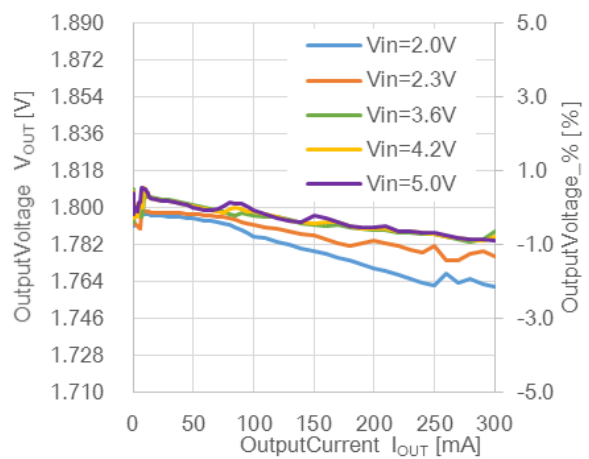
RP515x181x, Ta=25°C
