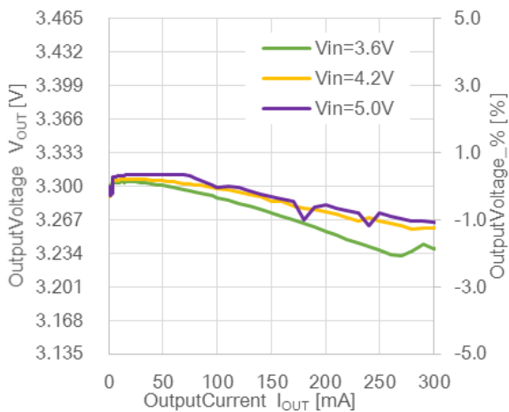
RP515x331x, Ta=25°C
