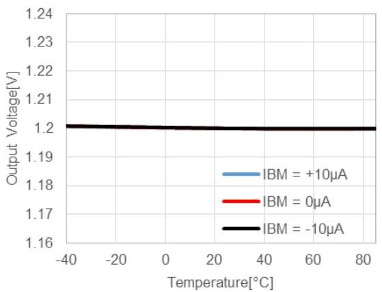
13) BM Output Voltage vs Temperature ( C_{OUT2} = Ceramic 0.1 \mu F, T_a = 25 ^{\circ} C) RP515xxx3x RP515xxx4x
