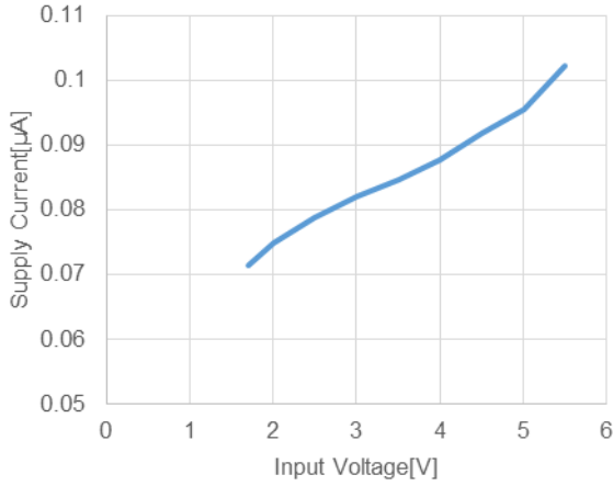
11) BM Supply Current vs Input Voltage ( C_{OUT2} = Ceramic 0.1 \mu F, T_a = 25 ^{\circ} C) RP515xxx3x RP515xxx4x
