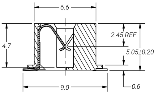
SECTION X-X
