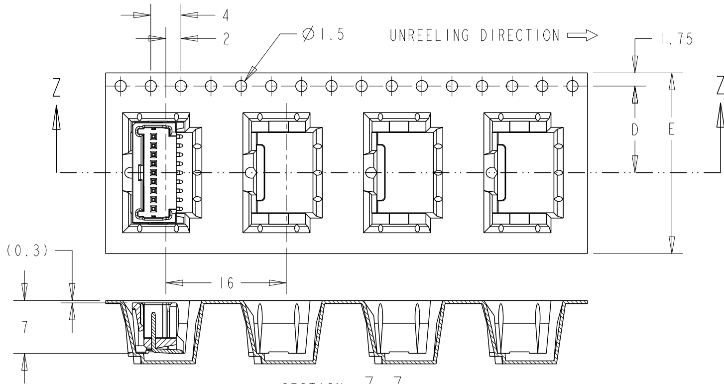
SECTION Z-Z TYPE 1 (2POS~9POS)
