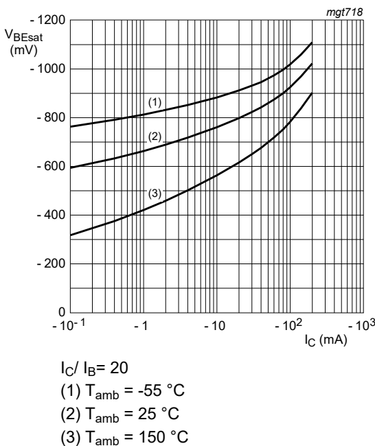
Fig. 11. BC857BQC: Base-emitter saturation voltage as a function of collector current; typical values
