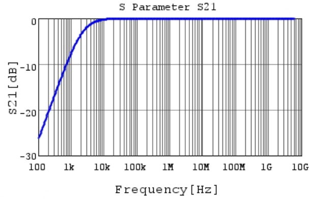
GRM155C70J105KE11 S21 DC0V, 25degC
