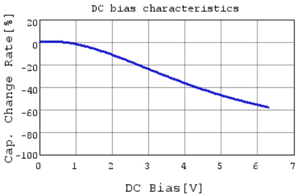
GRM155C70J105KE11 C-DC bias capchange, 25.0c
