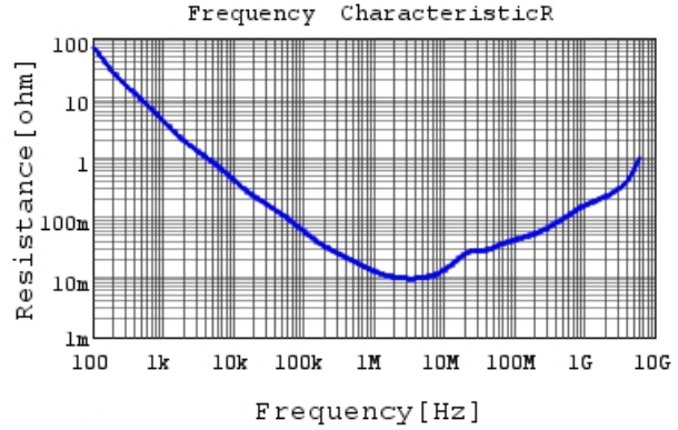
GRM155C70J105KE11 R DCOV, 25degC
