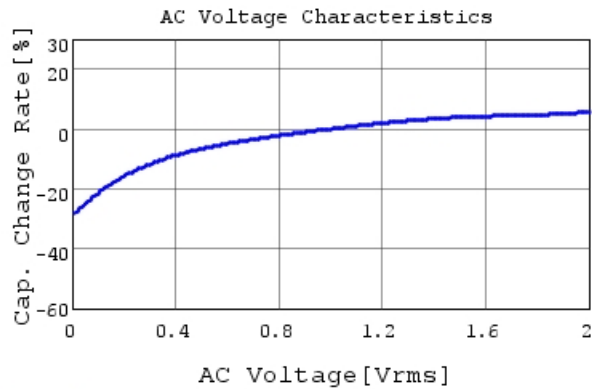
GRM155C70J105KE11 C-AC Voltage capchange, Dc
