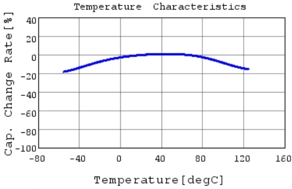
GRM155C70J105KE11 C-Temp. capchange, DC0.0V,
