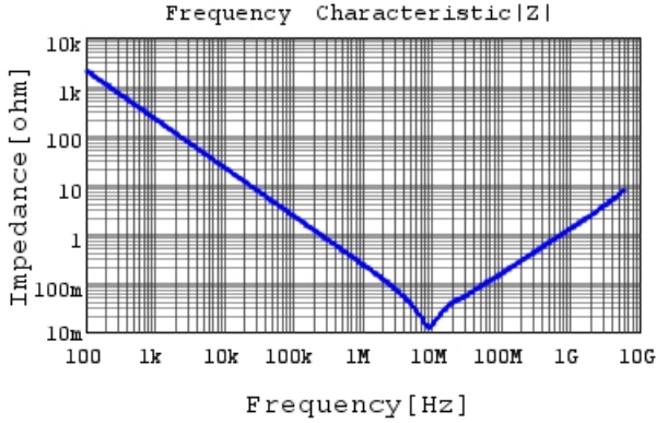
GRM155C70J105KE11 |Z| DCOV, 25degC
