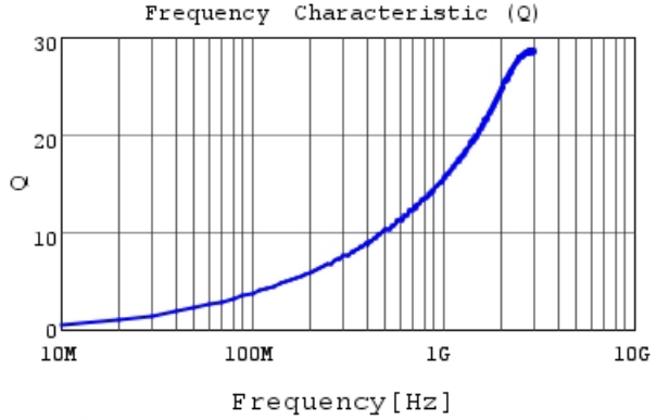
LQP02TN0N5B02 Q
