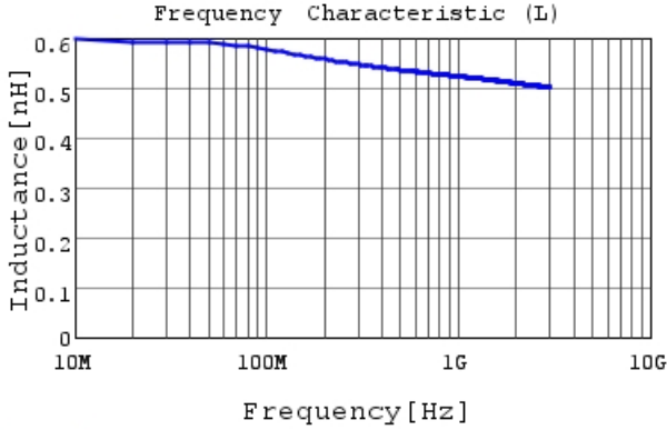
LQP02TN0N5B02 L
