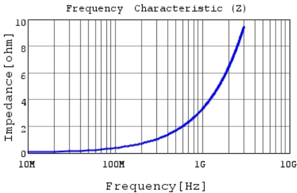
LQP02TN0N5B02 |Z|
