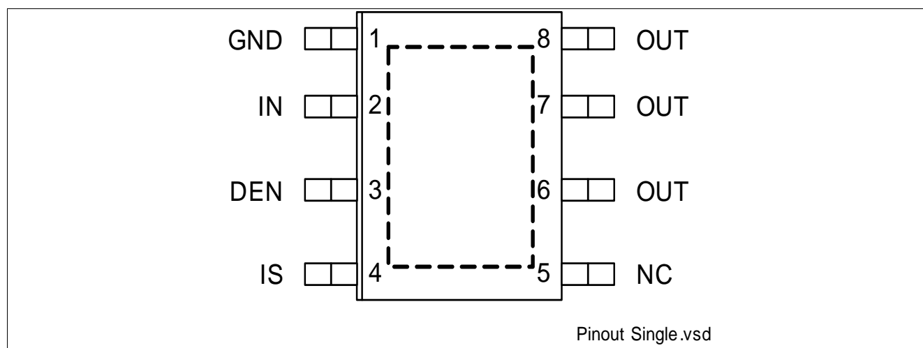
Figure 2 Pin Configuration
