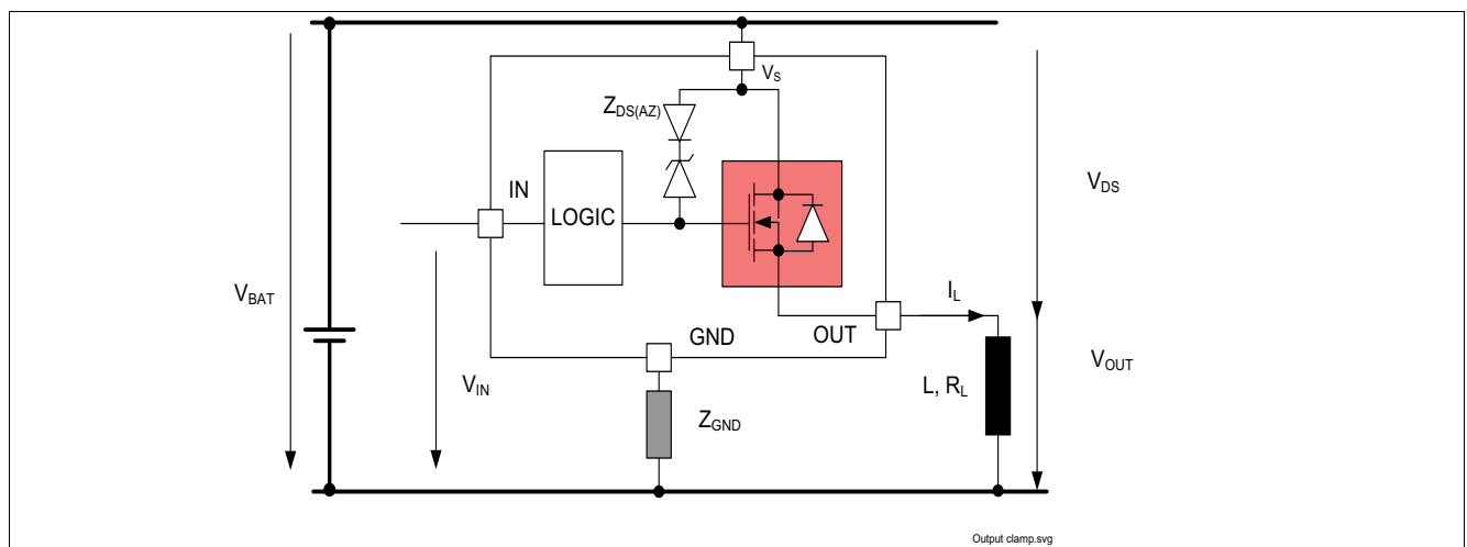
Figure 10 Output Clamp
