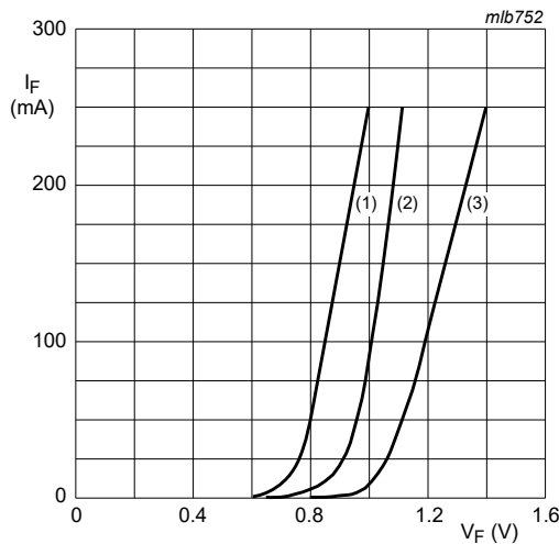
(1) T_{amb} = 150\text{ }^\circ\text{C} ; typical values (2) T_{amb} = 25\text{ }^\circ\text{C} ; typical values (3) T_{amb} = 25\text{ }^\circ\text{C} ; maximum values Fig. 2. Forward current as a function of forward voltage; per diode
