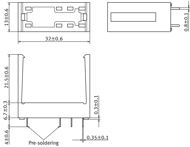
External dimensions
