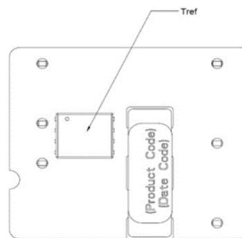
Figure 16. T_{ref} Temperature Measurement Location.
