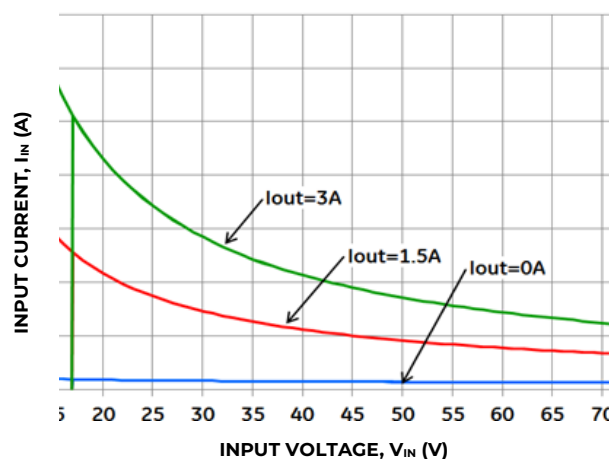
Figure 2. Converter Input Current versus Input Voltage.
