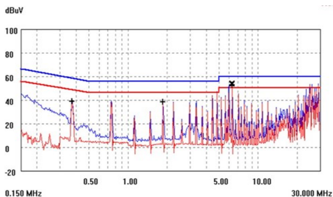
Figure 18. EMC signature using above filter.
