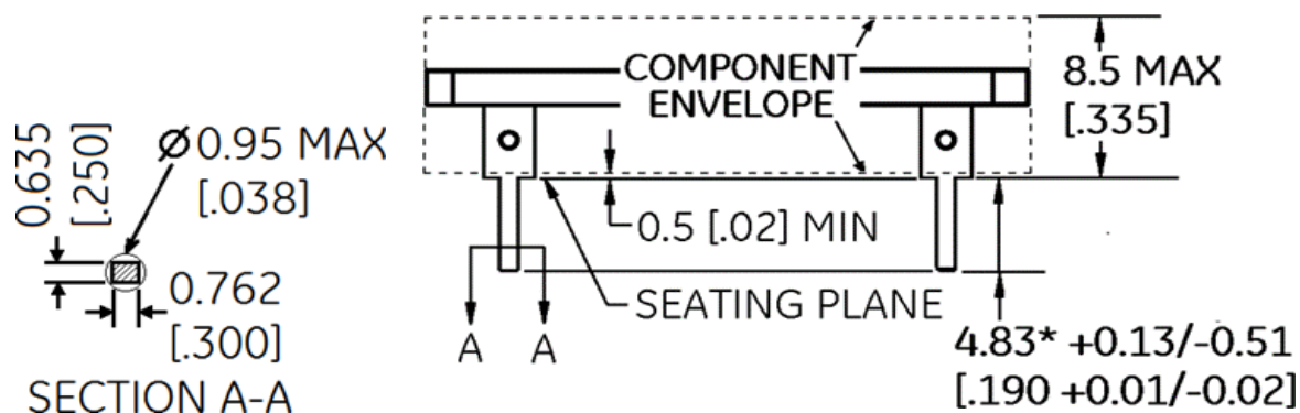
Side View
