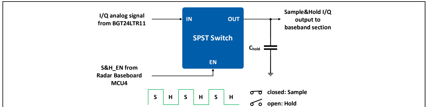
Figure 9 S&H circuitry
