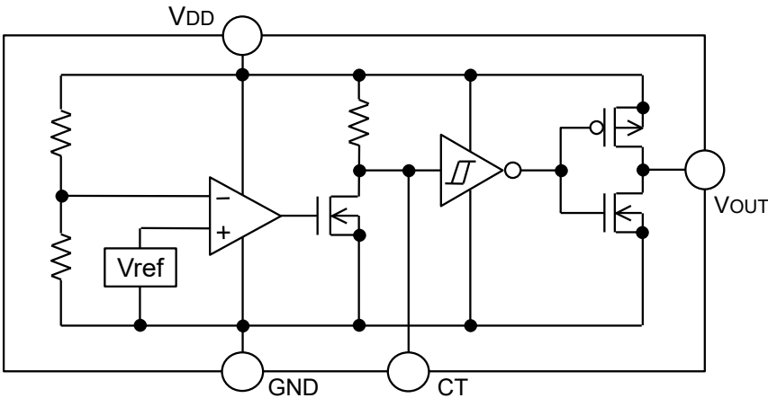
Fig.2 BD53xx Series
