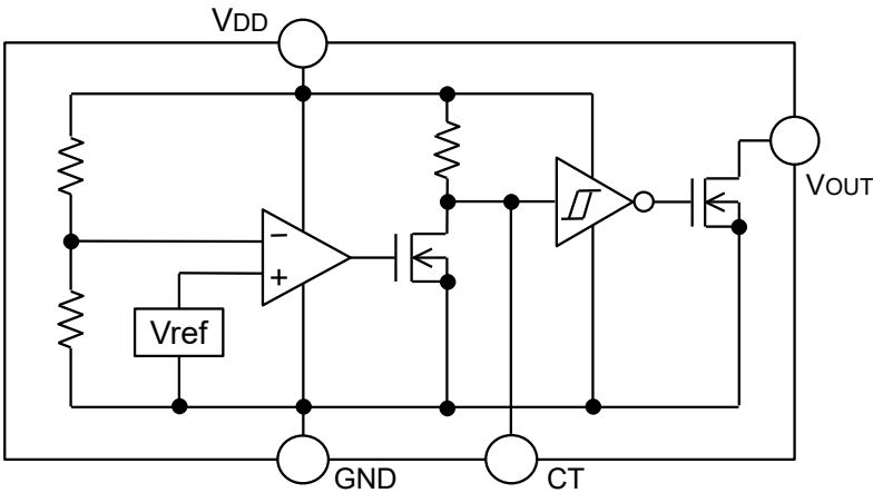
Fig.1 BD52xx Series
