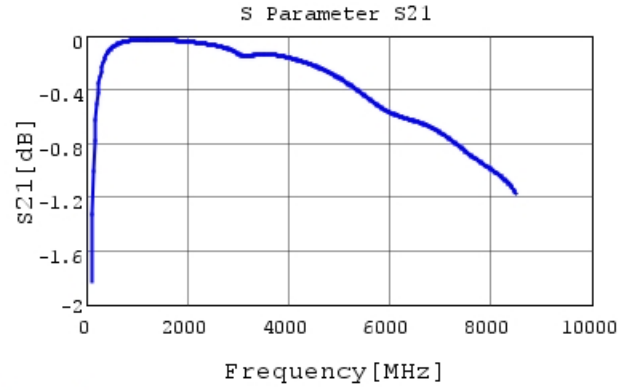
GRM1885C1H220JA01 S21 DCOV, 25degC
