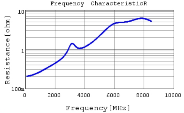
GRM1885C1H220JA01 R DCOV, 25degC
