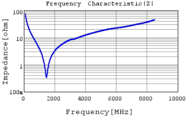
GRM1885C1H220JA01 |Z| DCOV, 25degC
