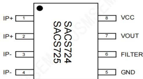
Pinout Diagram
