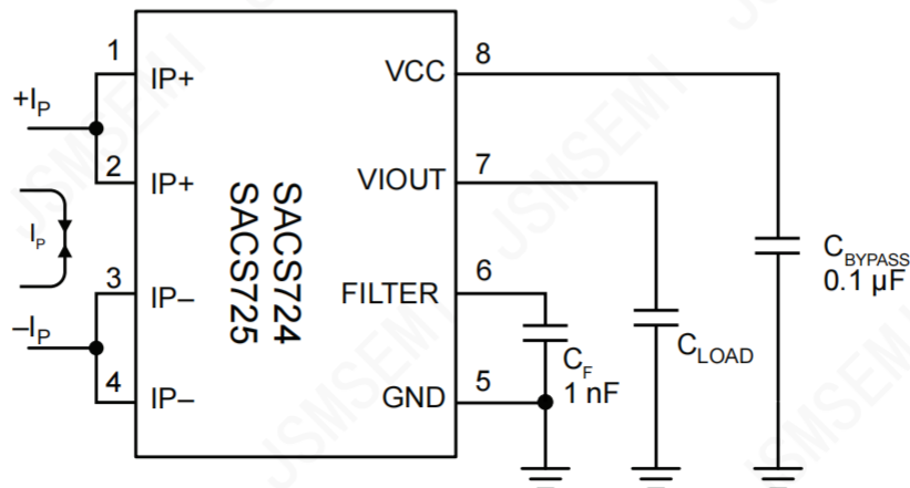
Figure 1. Typical Application Circuit Diagram
