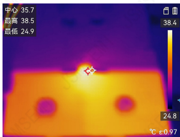
Figure 6. Thermal performance of 20A
