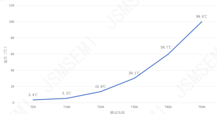
Figure 4. Thermal curve
