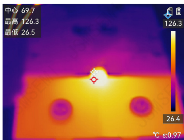
Figure 8. Thermal performance of 50A
