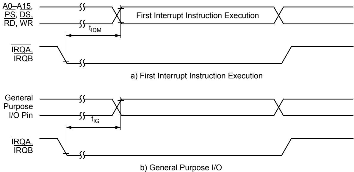
Figure 3-16 External Level-Sensitive Interrupt Timing
