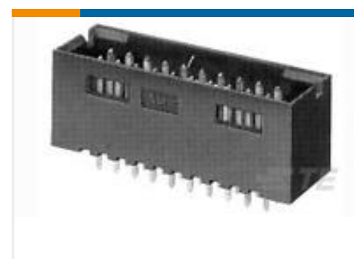
TE Part #5-103169-7 18 MODII HDR DRST SHRD .100CL
