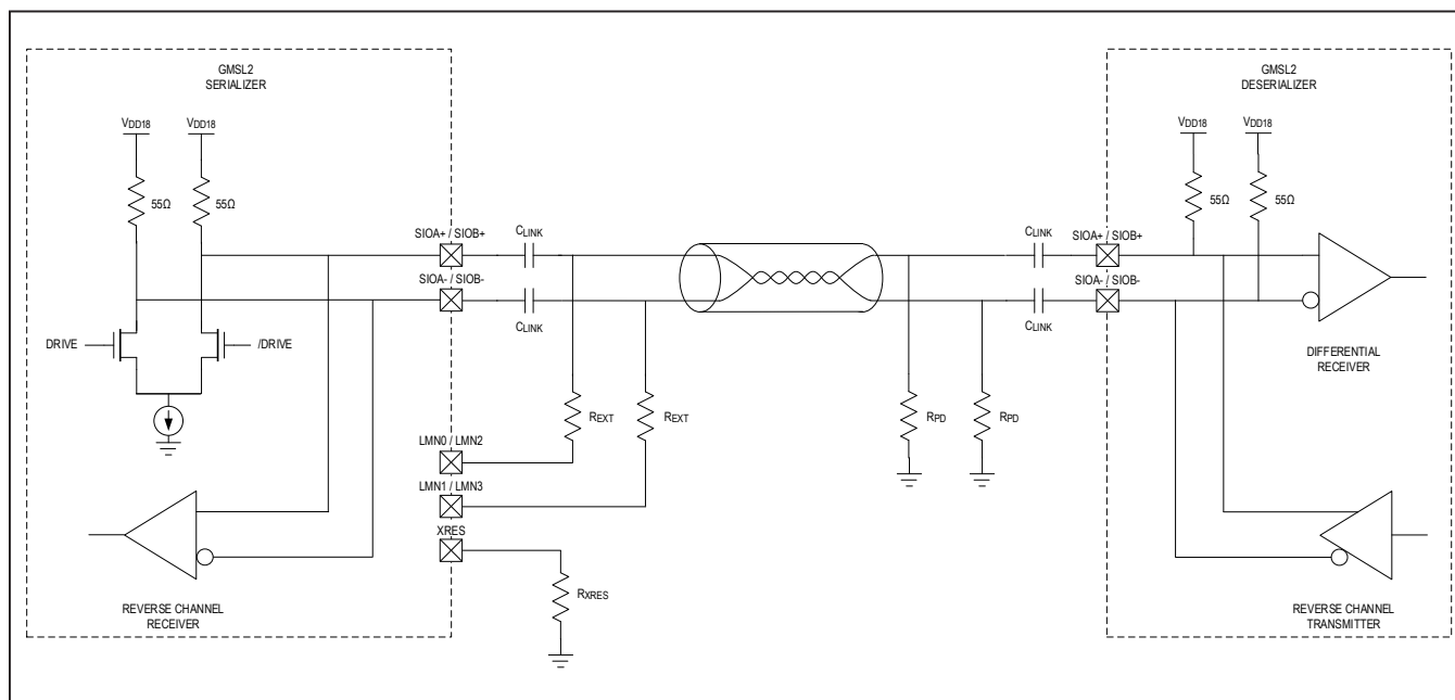
Figure 26. Line Fault Detection Connection for STP Cable
