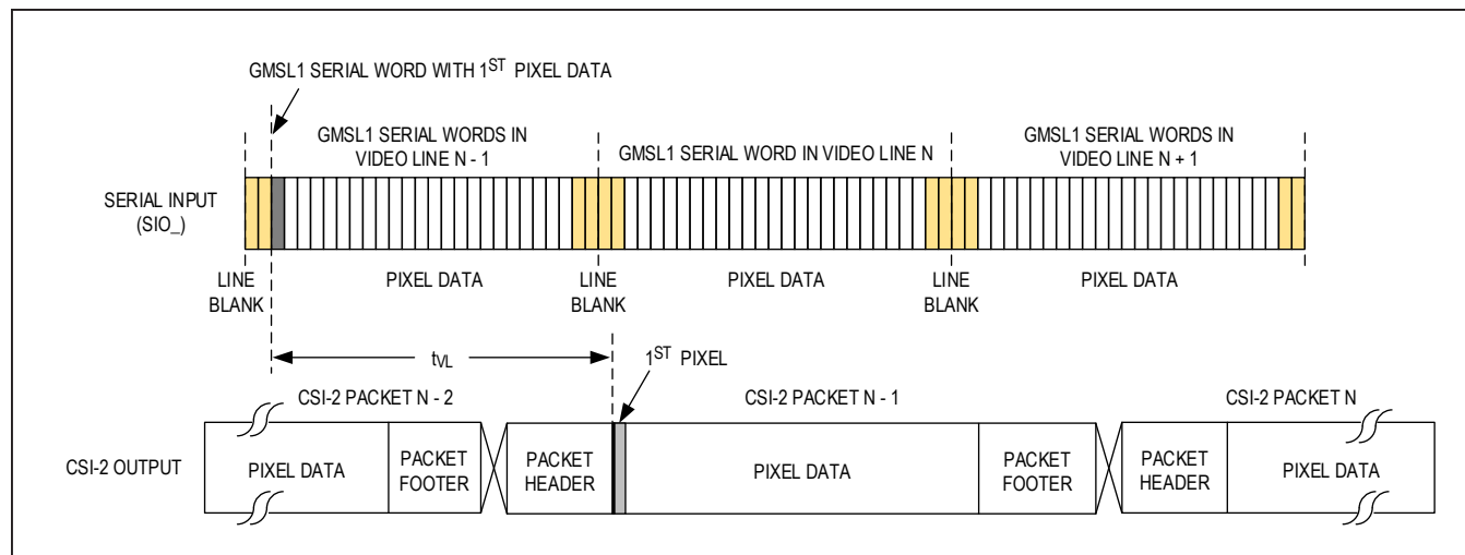
Figure 10. GMSL1 Video Latency
