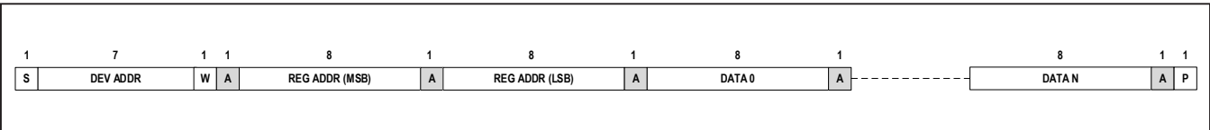
Figure 29. I 2 C Write Packet Format
