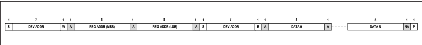
Figure 30. I 2 C Read Packet Format
