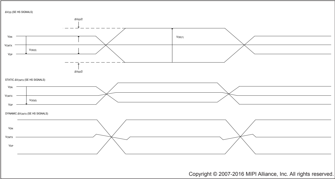
Figure 4. Possible Delta V_{CMTX} and Delta V_{OD} Distortions of Single-Ended HS Signals
