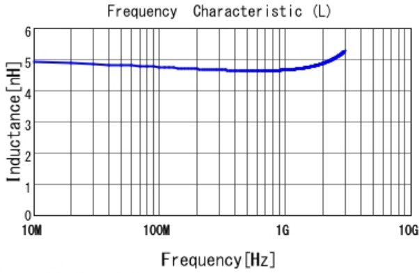
LQP03HQ4N7J02 L
