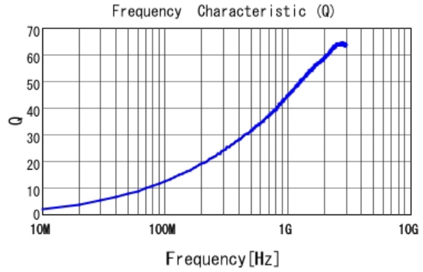
LQP03HQ4N7J02 Q
