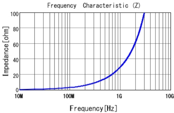
LQP03HQ4N7J02 |Z|
