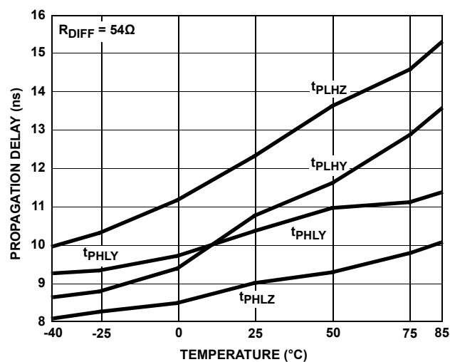
FIGURE 12. DRIVER PROPAGATION DELAY vs TEMPERATURE
